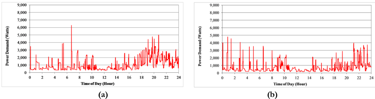
Figure 1 (a) Daily electrical profile – Winter (February) (b) Daily electrical profile – Summer (August)
