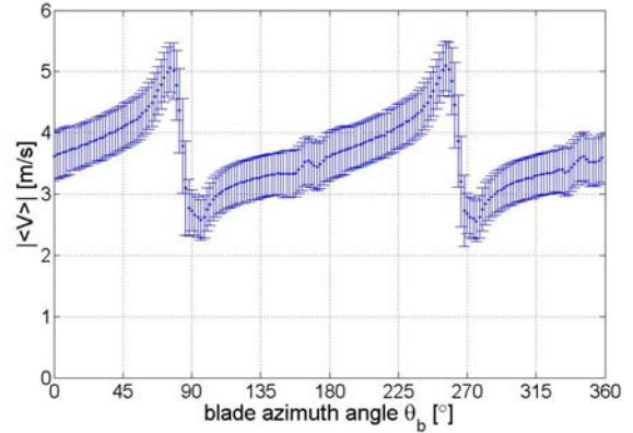
Figure 8. |\langle \overline{V} \rangle| versus \theta_b , including the total random uncertainty interval, for (r, \theta, z) = (0.42 \text{ m}, 270^\circ, 0.06 \text{ m}) . Blade passage: \theta_b \approx 90^\circ, 270^\circ , wake passage: \theta_b \approx 180^\circ, 360^\circ .
