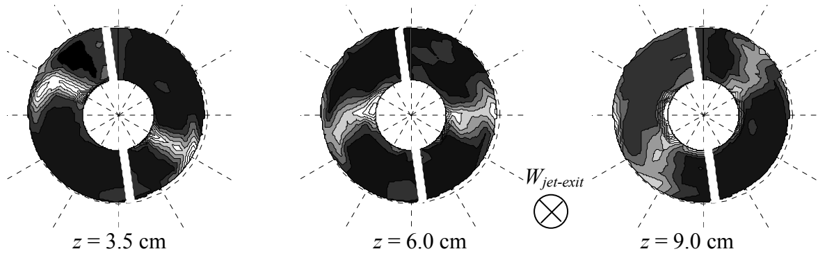
Figure 14. Contour plots of standard deviation s_{v_{eff}}(r, \theta, z, \theta_b) at \theta_b = 172^\circ , at downstream planes z = 3.5, 6.0 and 9.0 cm, for \Psi = 0^\circ . The two blades, indicated in white, rotate clockwise. \overline{W_{jet-exit}} is directed away from the observer. Going downstream, the wake diffuses and the relatively straight shape, observed at z = 3.5 cm, deforms.
