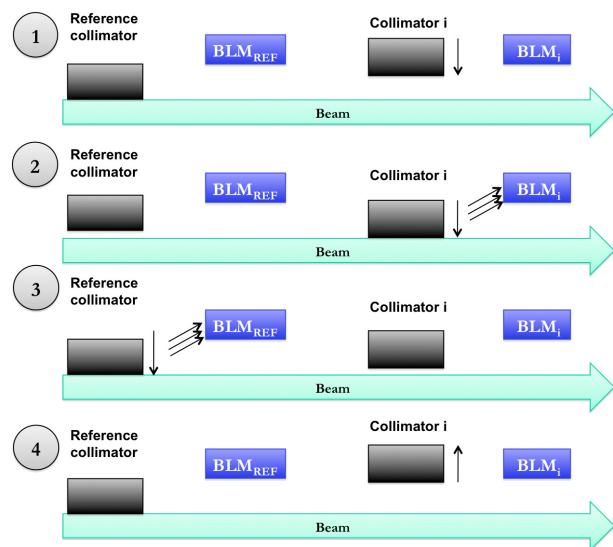
Figure 1: Setup Sequence.
