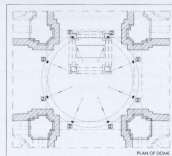
PLAN OF DOME
