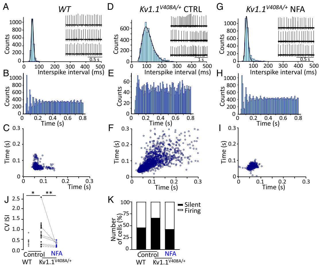
Fig. 4. NFA ameliorates the firing properties of Purkinje cells recorded from Kv1.1^{V408A/+} mice. Representative ISI distribution (A), spike recording (Inset), ISI autocorrelation (B) and scatter plot (C) constructed for a PC recorded extracellularly from a cerebellar brain slice of a WT mouse and, respectively, for a sample Kv1.1^{V408A/+} PC recorded and analyzed before (Control, CTRL) (D–F), and after the superfusion of 100 \mu M NFA (G–I). Note that the ISI distributions were fitted with a probability density function of the exponentially modified Gaussian distribution with variance values of 8.7 for WT (A), 45 for Kv1.1^{V408A/+} /CTRL (D), and 15 after NFA treatment (G). (J) CV ISI calculated for WT and Kv1.1^{V408A/+} PCs (* P < 0.01 ; unpaired t test). The latter PCs were recorded before (Control) and after NFA (100 \mu M) application (mean \pm SEM; ** P < 0.001 ; unpaired t test). Note that Kv1.1^{V408A/+} PCs displayed an irregular firing compared to WT, which was ameliorated by NFA treatment. (K) Percentage of silent (black bar) or spontaneously firing (white bar) PCs recorded from WT and Kv1.1^{V408A/+} mice before (Control) and, upon incubation with NFA (100 \mu M). The NFA-induced increase in the percentage of spontaneously firing PCs was statistically significant: * P < 0.01 , ** P < 0.001 unpaired t test.
