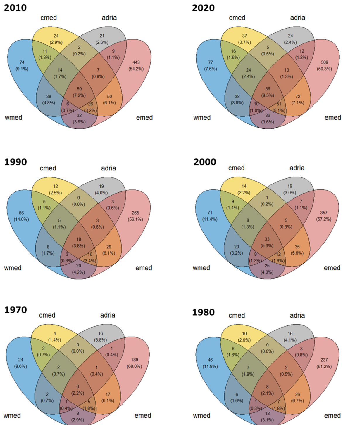
Figure 4. Cumulative number of species that are unique to or shared between the four Mediterranean subregions at a decadal scale between 1970 and 2020. Each intersection in the Venn diagrams represents the number (percentages in parentheses) of species contained only within the specific combination of geographic areas and nowhere else. wmed = western Mediterranean, cmed = Central Mediterranean and the Ionian Sea, adria = Adriatic Sea, emed = eastern Mediterranean.
