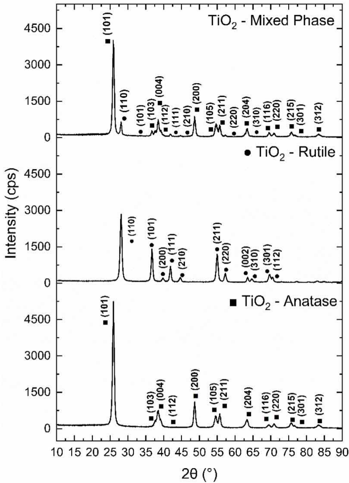
Figure 1. XRD diffractograms of samples compared with DB cards of the anatase, rutile, and anatase-rutile mixed phase
