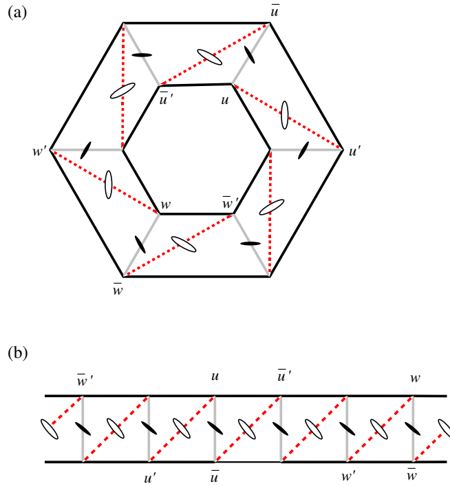
Figure 4. Construction of sign-unbalanced regular nut graphs with degree n - 2 . The graphs \Gamma(G, \Sigma) are based on cocktail-party graphs G = CP(2p) where 2p is divisible by 4. (a) Schlegel and (b) unfolded-net representations of the graph \Gamma = (CP(12), \Sigma) in a prism setting of the chiral point group D_6 . Black- and white-filled symbols indicate points where two-fold rotational axes enter and leave the prism. Axis C'_2(u) enters the prism midway between vertex u and its graph-antipodal partner \bar{u} , to emerge between vertex w and its graph-antipodal partner \bar{w} . Axis C''_2(u) enters the prism between vertex u and its neighbour on a negative edge u' , to emerge between vertices w and w' . Dashed lines denote the edges with weight -1 , chosen as described in the proof of Theorem 20. Grey lines denote the ‘missing edges’ deleted from the complete graph K_{2p} . Solid black lines denote edges of weight +1 , though not all are shown: the graph has an edge of weight +1 connecting each vertex w with all vertices other than \bar{w} , w' and w itself.
