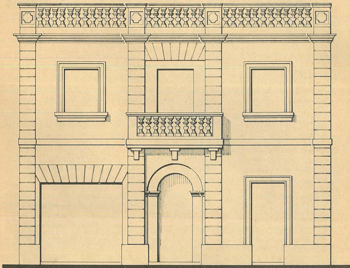
ELEVATION. DOMUS CURIALIS, ŻEJTUN.
