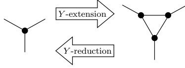
Figure 3: Y-operations
