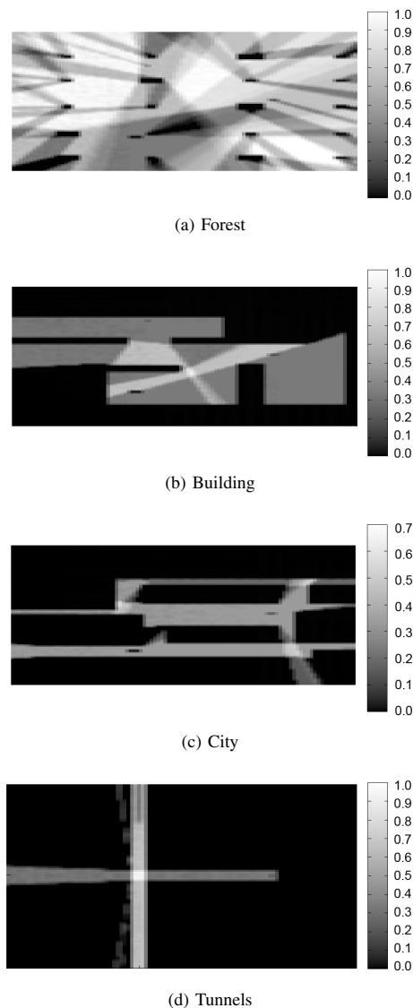
Fig. 3: Top-down view of the fitness landscapes of the four testbeds. The sample is calculated setting the camera position at a height of one meter from the ground level of the maps, This corresponds to half the height of the virtual character.
