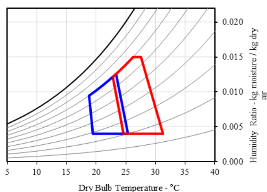
Figure 3: Local thermal comfort zones with 90% acceptability.
