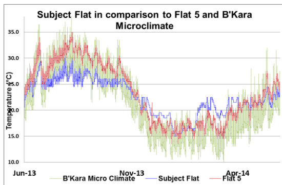
Figure 6: Temperature comparison between the subject flat (blue), flat 5 (red) and B'Kara microclimate (green).
