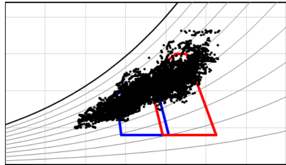
Figure 8: Retrofitted Subject Flat DesignBuilder Indoor Climatic Data with 90% TCZs.
