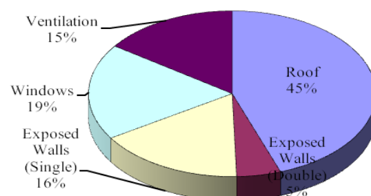
Figure 1: Steady state heat transfer model of the subject flat prior to renovation.
