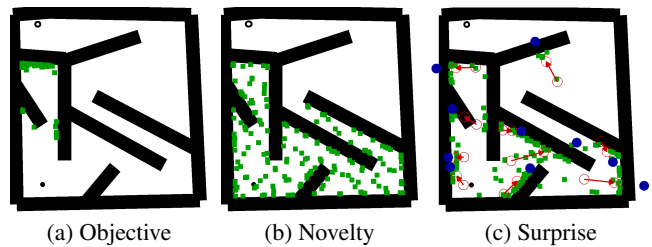
Figure 2: The process of different types of search for maze navigation on the “hard” maze of Lehman and Stanley (2011a). The solid black circle (bottom left) is the starting position, and the empty black circle (top left) is the goal; green dots represent the agents. For surprise search (Fig. 2c), red circles represent the population’s centroids of the two prior generations; the red arrow is the direction of the centroid, from the earliest generation to the latest generation, while the blue circles are the predictions for the clusters’ centroids in the current generation. Surprise search rewards the individuals in the current population (green) which deviate from the closest prediction point (blue).
