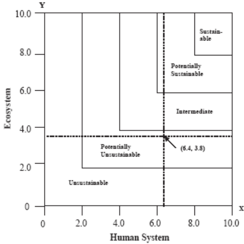
Figure 1: The BTS-model
