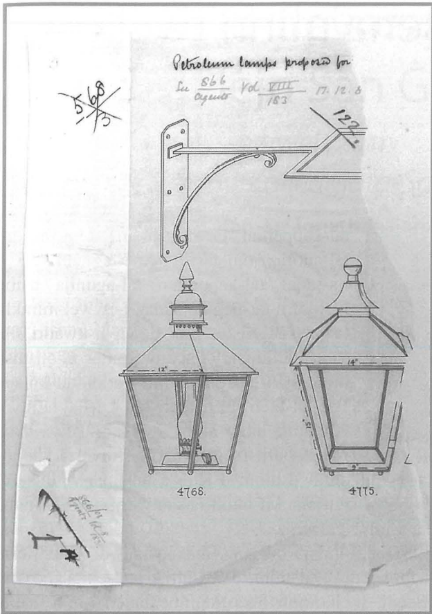
Id-disinn tal-fanali tal-pitrolju
