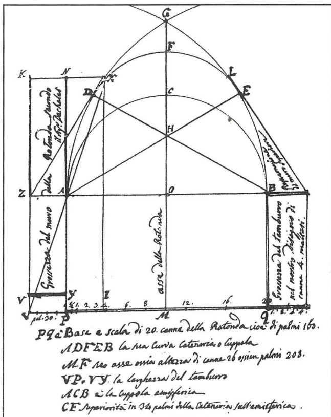
Wahda mid-disinj mhejjija minn Ġorġ Grognet de Vassè għar-rotunda. (mill-ktieb 'Grognet Confuta Fergusson' miktub minn Dun Edgar Salamone - 1910).
