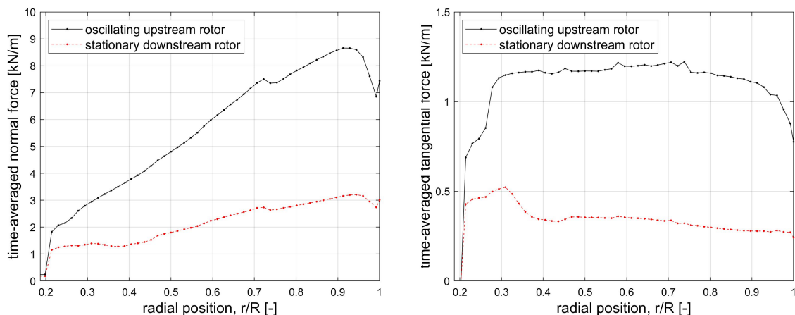
Figure 11: Spanwise distribution of normal and tangential loads for the oscillating upstream rotor (rotor 1) and the stationary downstream rotor (rotor 2) in the last time step.
