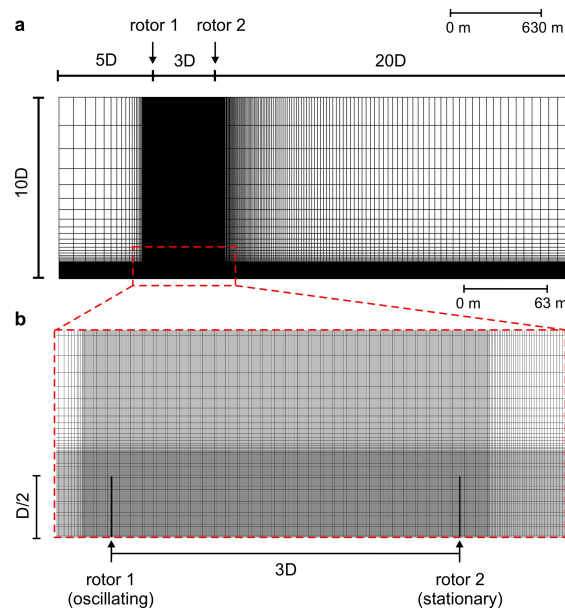
Figure 5: Computational domain and grid for the CFD simulation.
