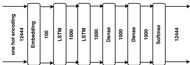
Figure 2: Word-based neural network architecture used in DeepTingle.
