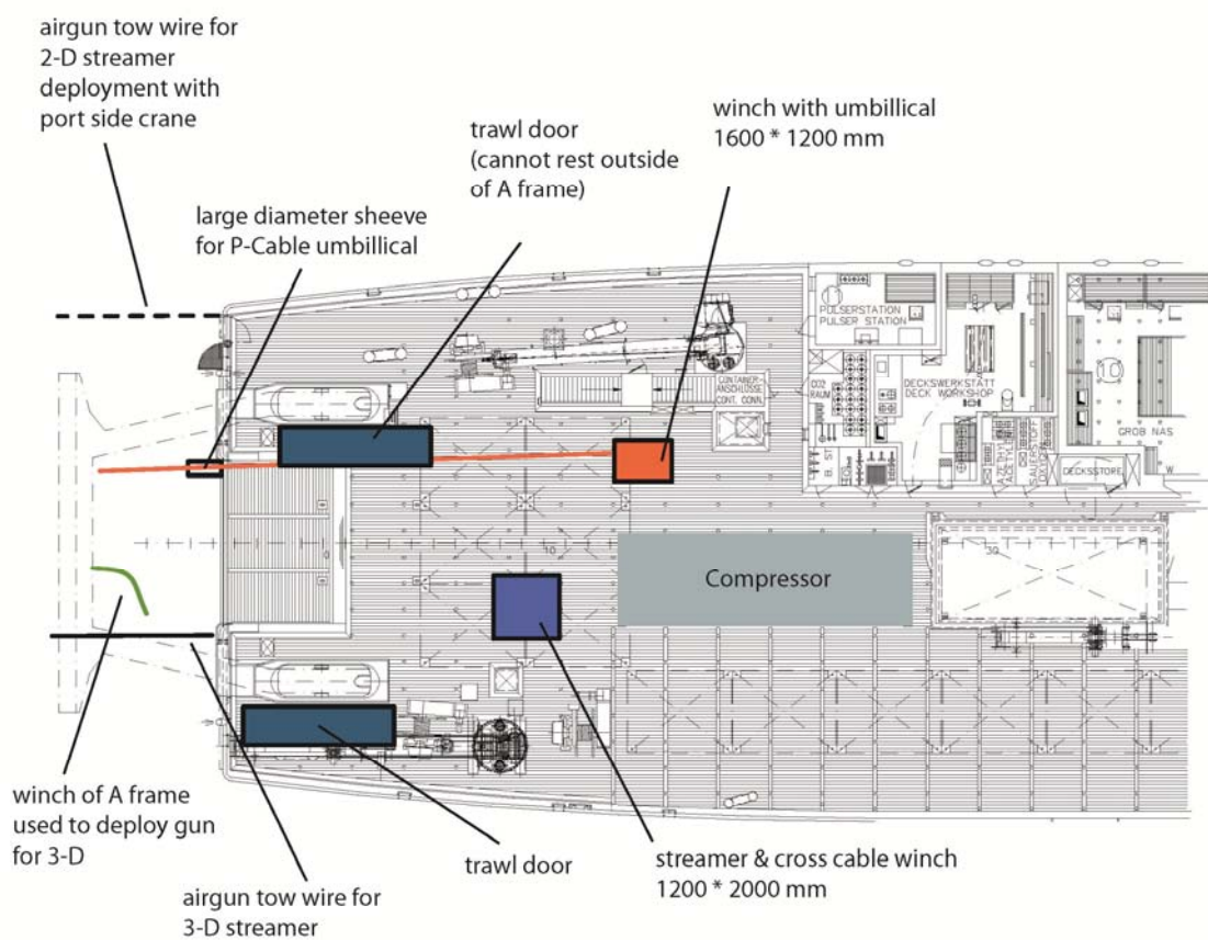
Fig. 23 Distribution of the seismic equipment on the aft deck of R/V METEOR during cruise M86-2.
