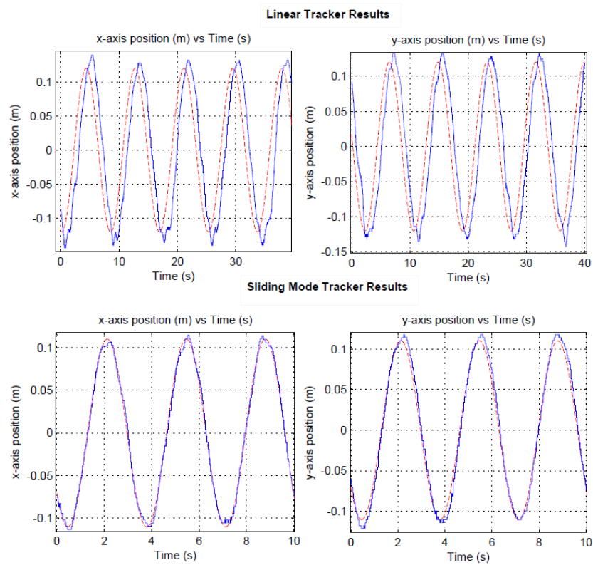
Experimental results for ball and plate setup
